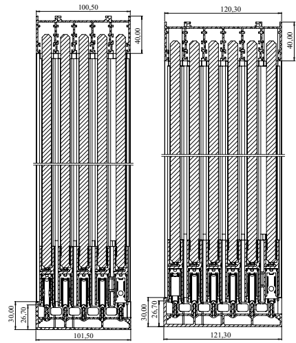
5 Railed Sliding System S
