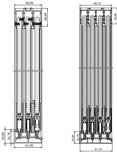
3 Railed Sliding System S
