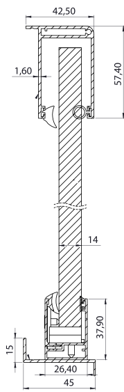
Plus Triangle Insulated Glass
